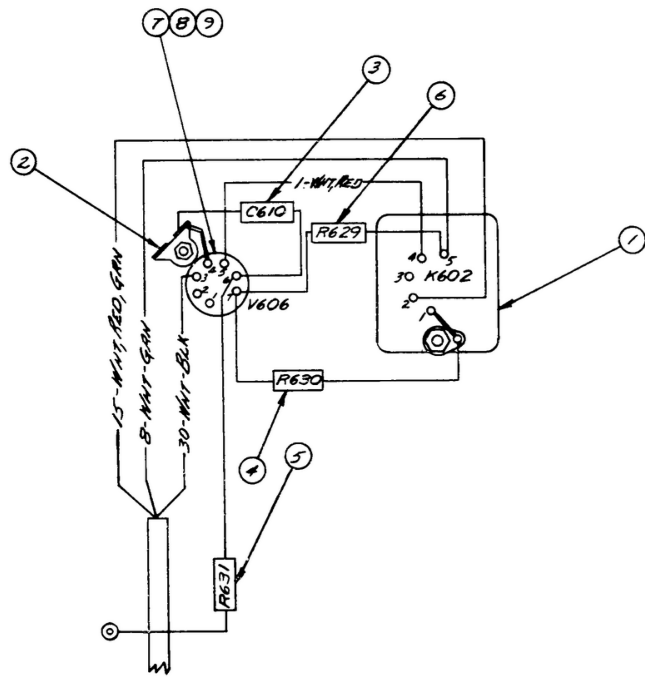
WIRING DIAGRAM - SQUELCH
